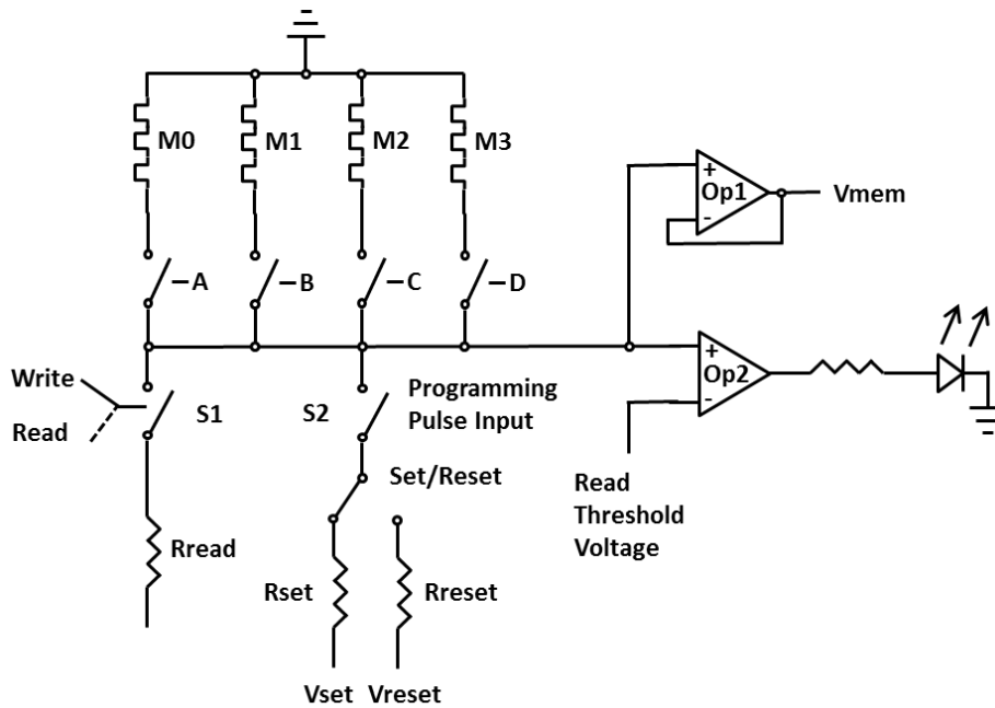
Figure 23. Pulse Mode Simplified Circuit
